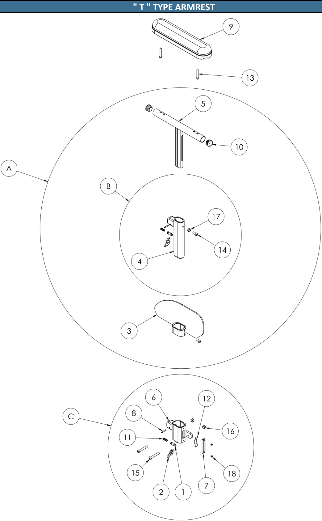
1 LEFT ASSEMBLY ILLUSTRATED
